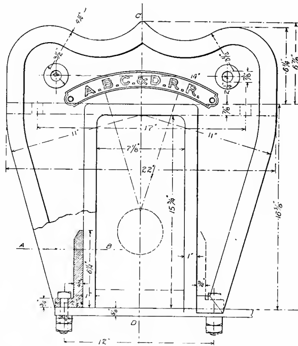
Fig. 5481. Sectional Elevation.
